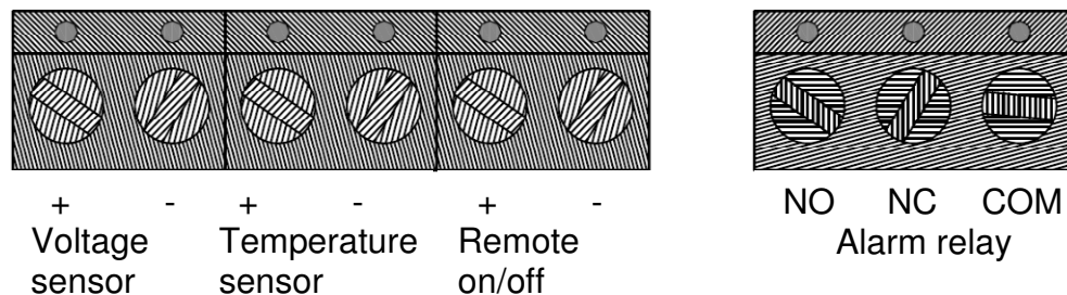
Figure 5 Connector block
